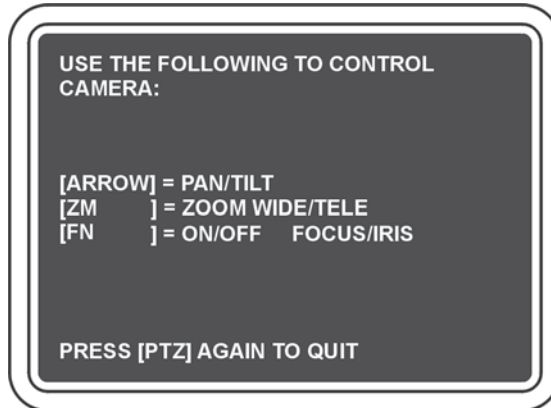
Figure 29. PTZ Instructions
