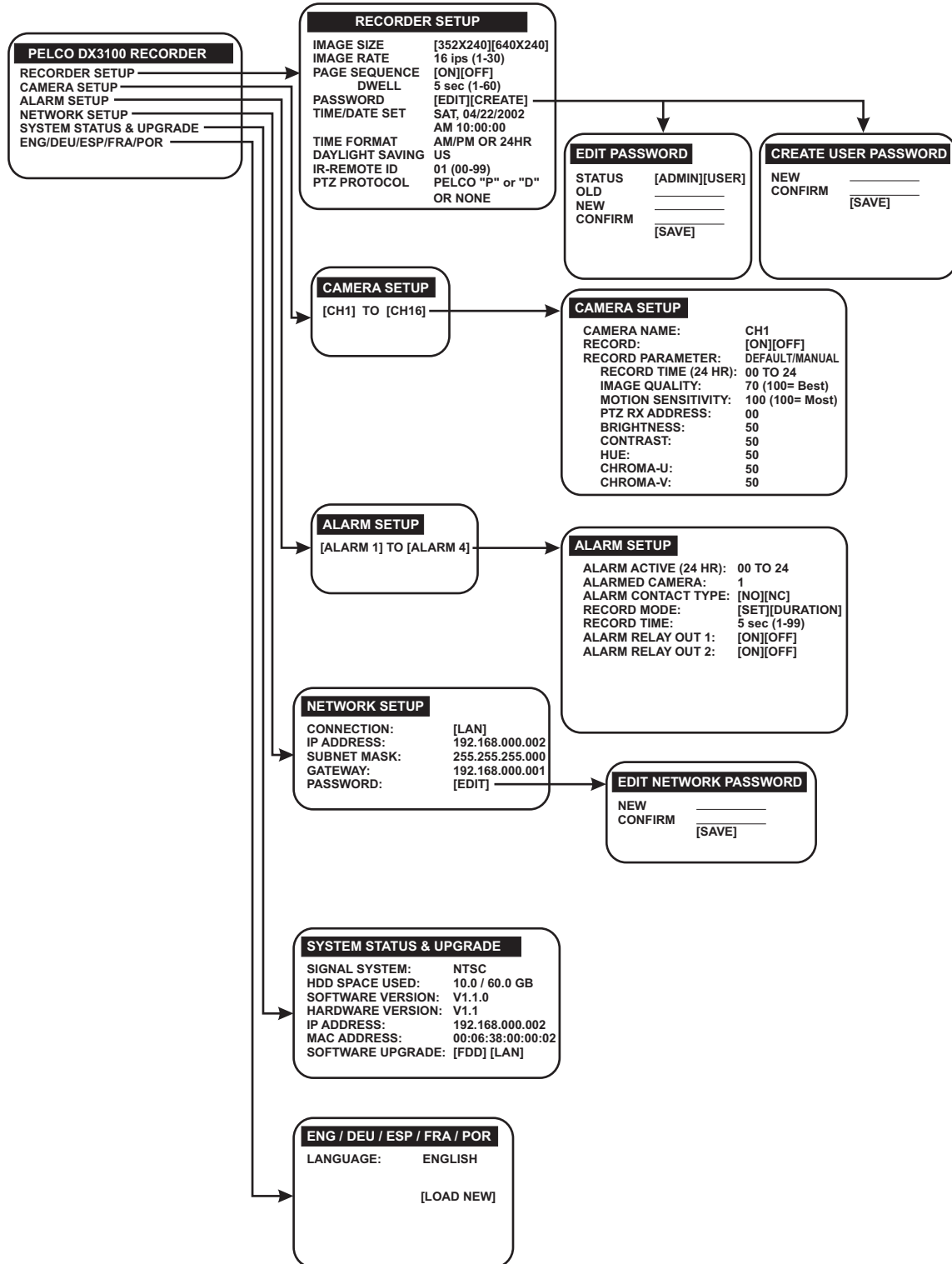
Figure 7. Menu Tree
