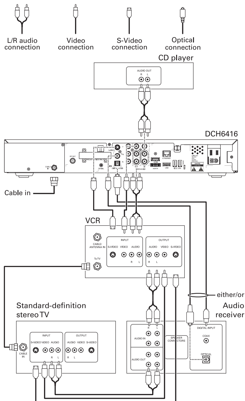
Figure 3-4 Cabling an audio receiver
