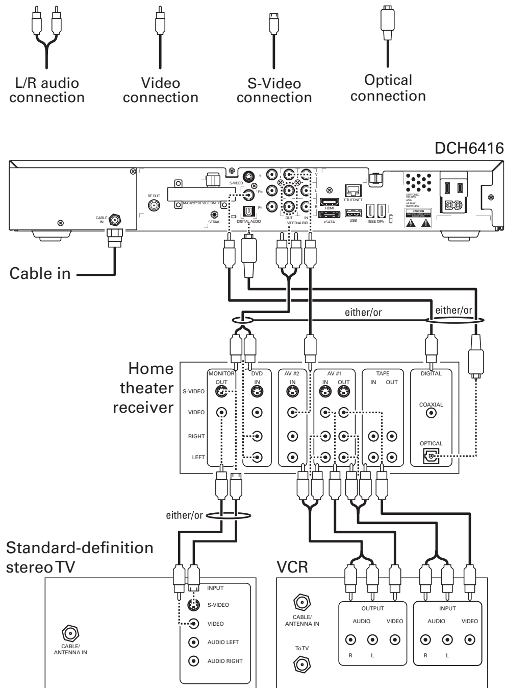
Figure 3-3 Cabling to a Standard-Definition stereo TV
