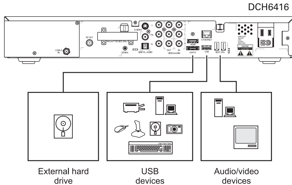
Figure 3-5 Sample data devices you can connect to the DCH6416
