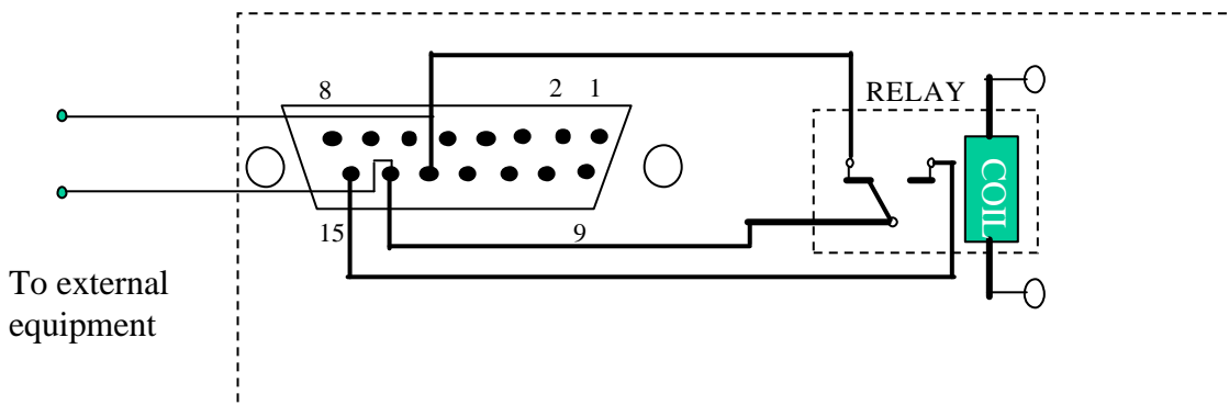
Normally Closed Connection (use pin # 13 and # 12)
