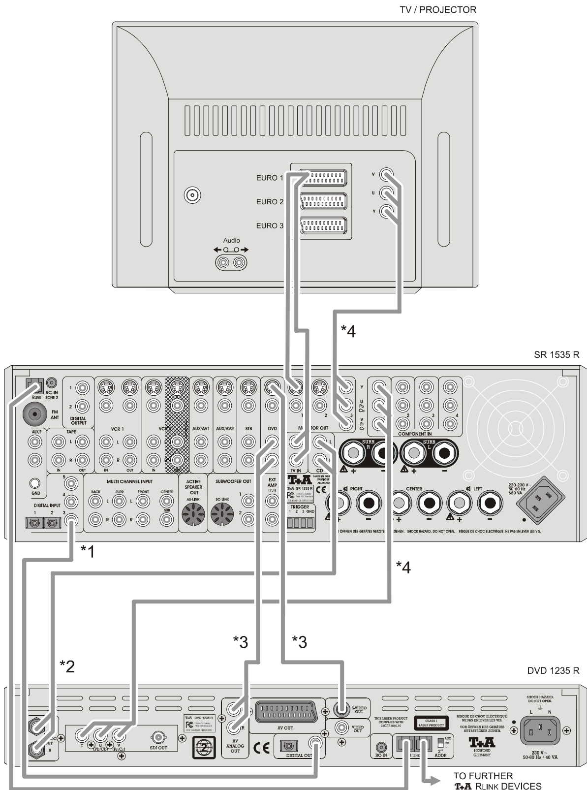
Wiring diagram 1: DVD 1235 R and SR 1535 R with S-Video and Component YUV Video
