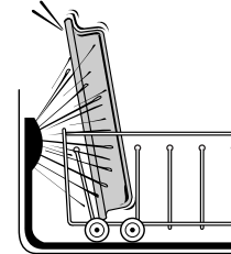
POWERSCOUR™ wash area side view
