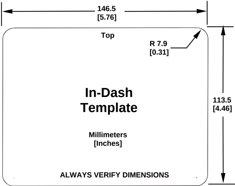
In-dash mounting template for the GlobalMap Baja 480c, showing dimensions. NOTE: The figure above is not printed to scale. A scaled template (FM-5 In-Dash Adapter Kit instructions) is available for free download from our web site, www.lowrance.com .
