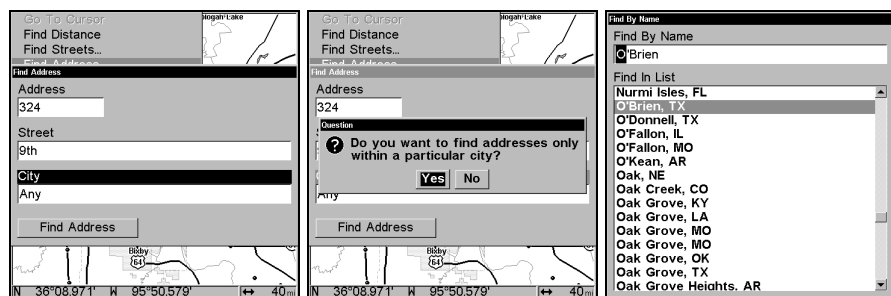
Find City field (left); Search in particular city option (center); Find City by name (right).
