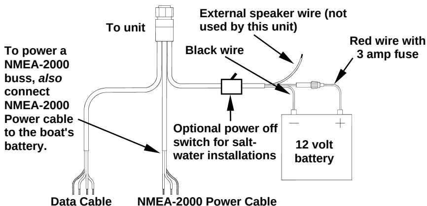
Power connections for the GlobalMap Baja 480c GPS unit.
