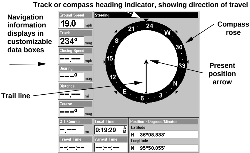
Navigation Page, recording a trail, traveling southwest. Page looks like this when the unit is not navigating to a waypoint, following a route, or backtracking a trail.
