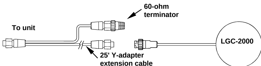
LGC-2000 Cable Connection.
