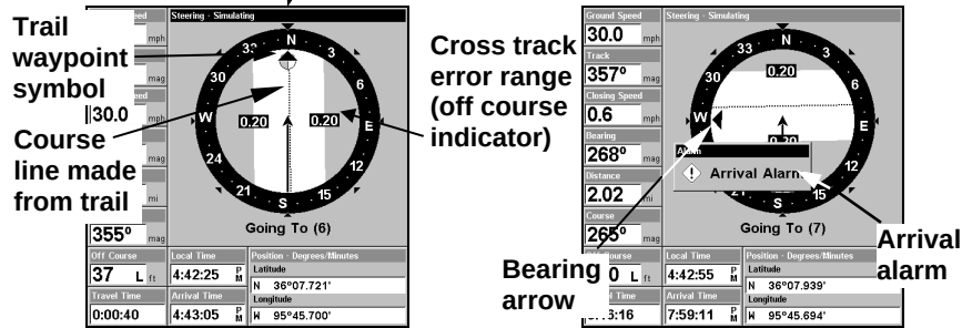
Navigate trail, navigation page (compass rose) views: driver (left) is northbound heading straight toward trail point 6; bearing arrow shows the trail point is due north (straight ahead.) driver (right) has reached trail point 6 and must turn west to follow the trail. Arrival alarm goes off and bearing arrow swings around to say turn left (west), toward the next waypoint, trail point 7. The unit now shows navigation information to point 7, which is 2.02 miles away.
