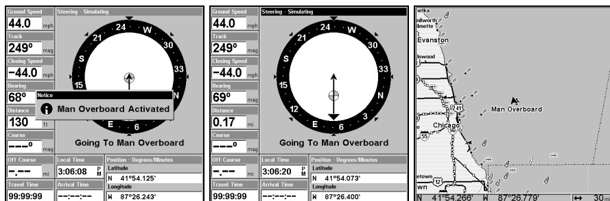
Navigating to Man Overboard: Man Overboard Activated message (left), Navigation Page (center); Map Page (right). The victim is to the starboard of the vessel. The GPS shows where to go for the rescue.
