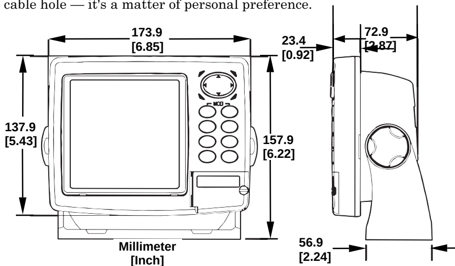
Front view (left) and side view (right) showing dimensions of the GlobalMap Baja 480c when mounted on gimbal bracket.
