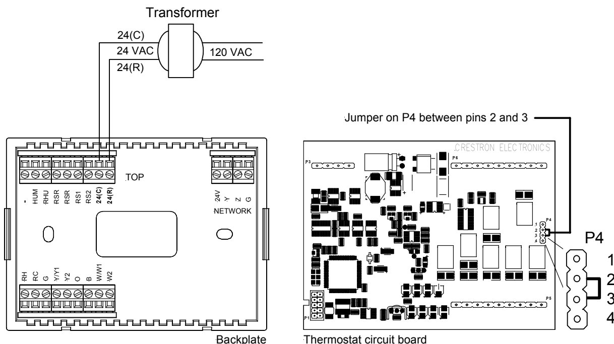
Backplate Connection and Circuit Board Jumper Position
