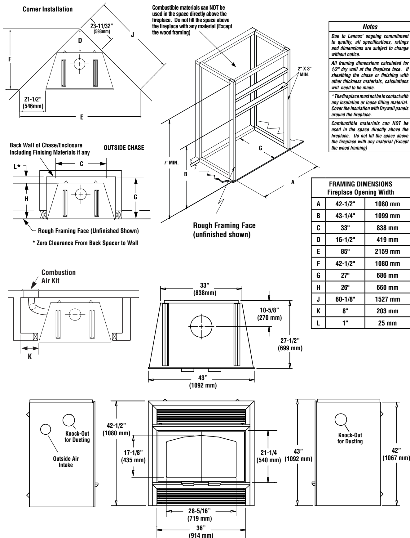
Figure 10 - Framing Dimensions
