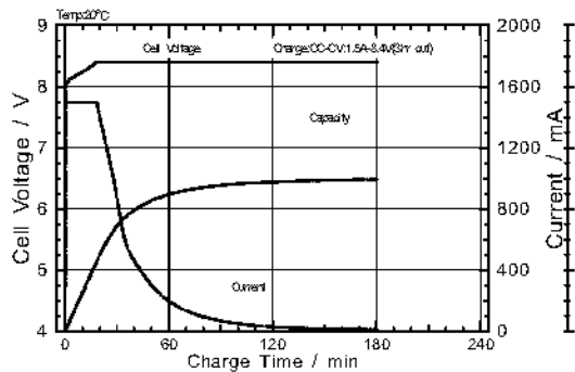
Charge characteristics
