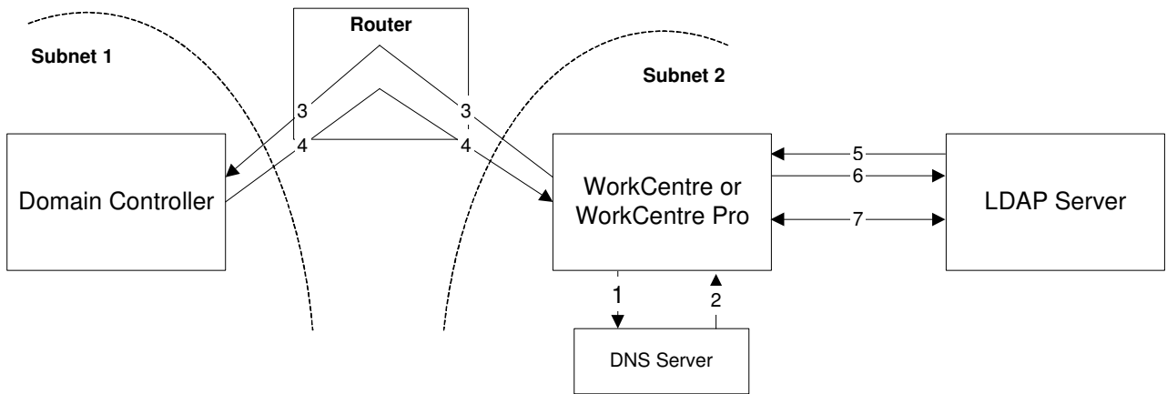
Figure 3-2 SMB Authentication with Hostname
