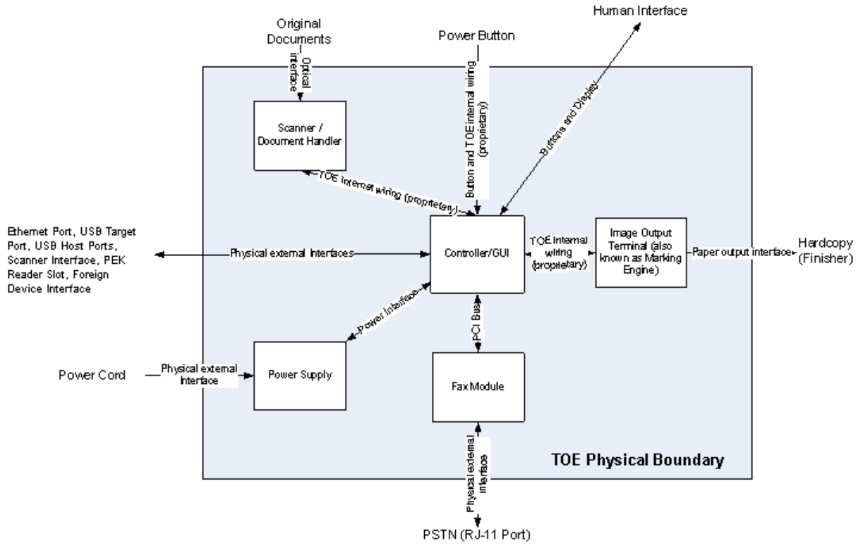
Figure 2-2 System functional block diagram
