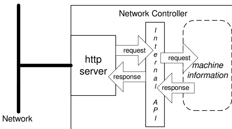
Figure 2-6 HTTP
