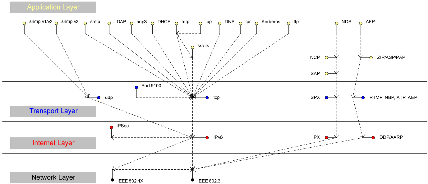
Figure 2-5 IPv6 Network Protocol Stack
