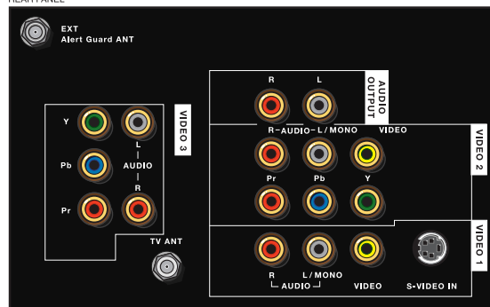
REAR PANEL
