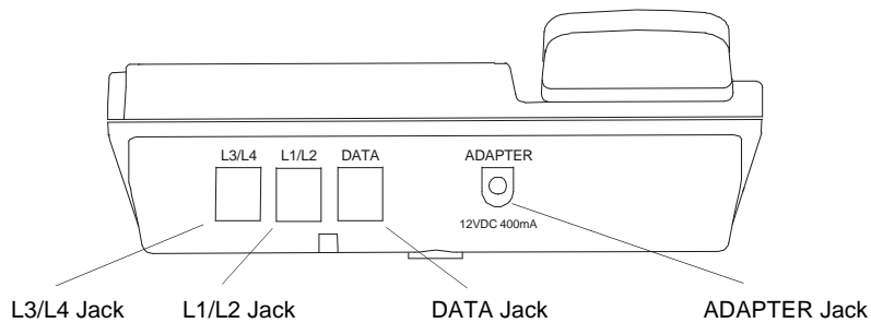
Model IBM-412 Rear View
