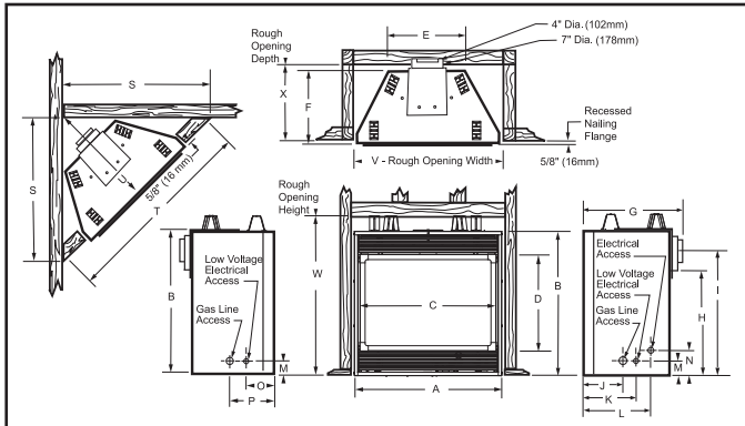
FIREPLACE DIMENSIONS - XDV (REAR VENT)
