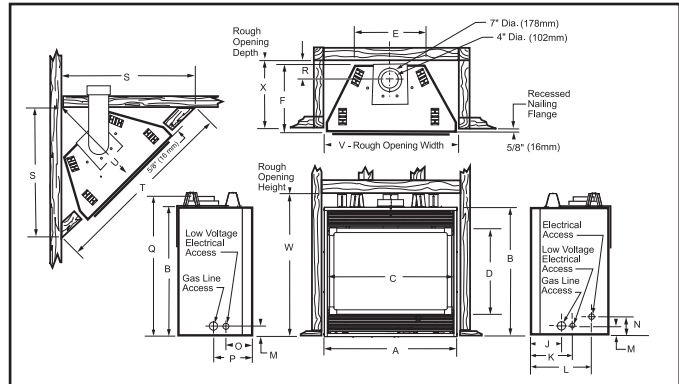
FIREPLACE DIMENSIONS - XDV (TOP VENT)
