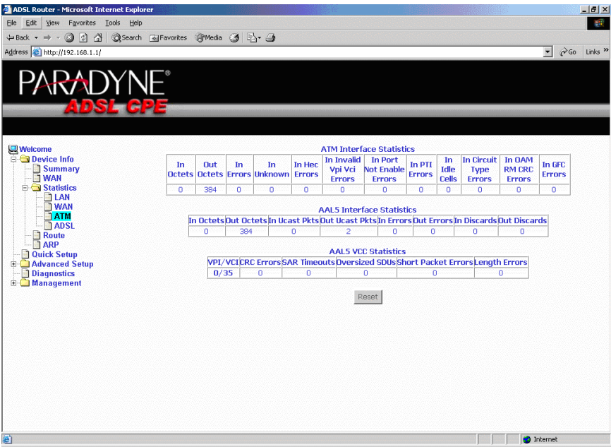
Figure 3-5. ATM Statistics
