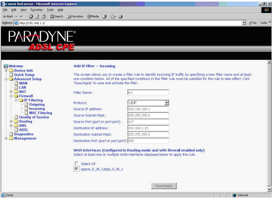
Figure 5-19. IP Filtering - Incoming Filter Add
