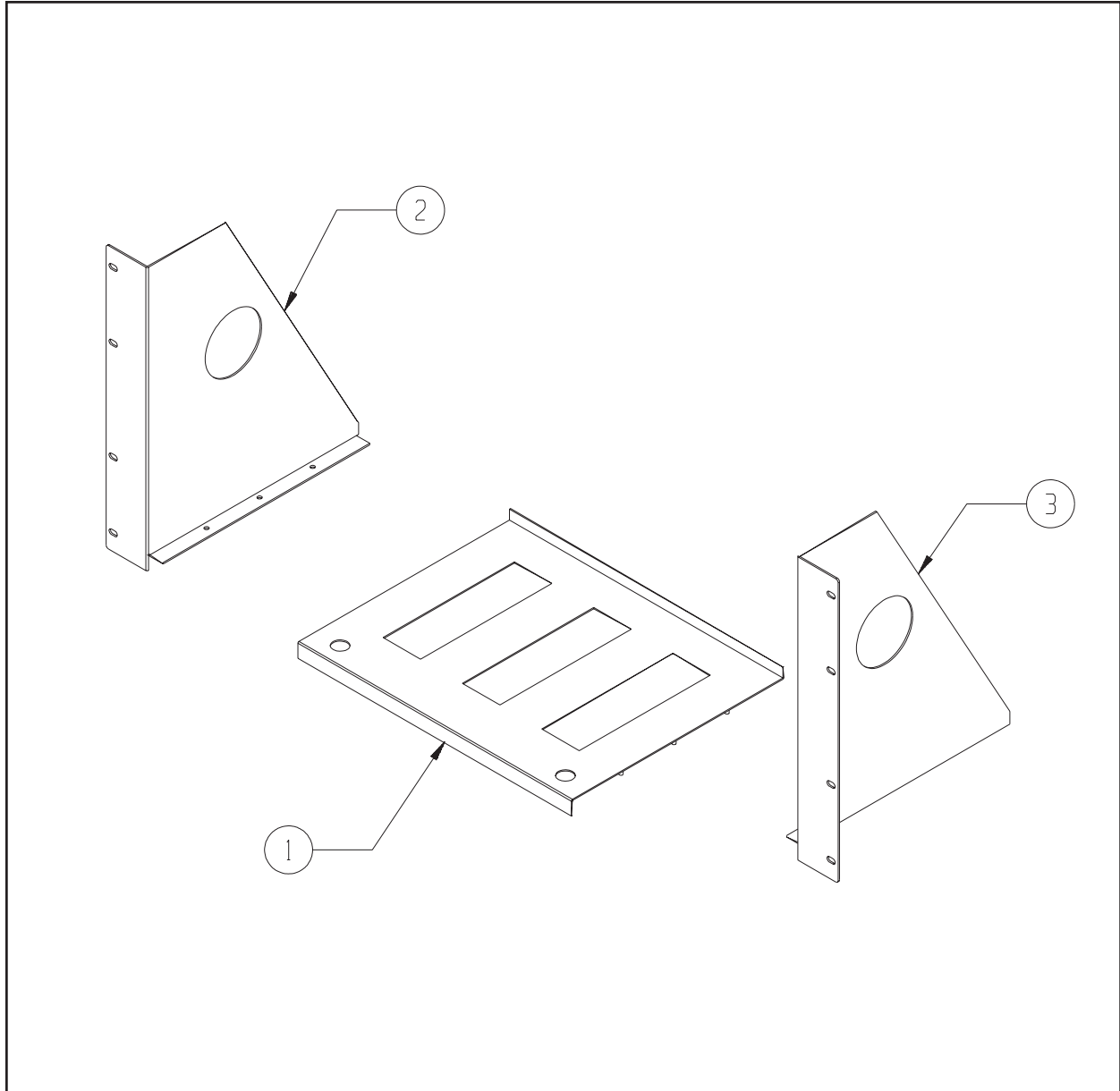
Figure 2. RMA131SU Rack Kit Assembly
