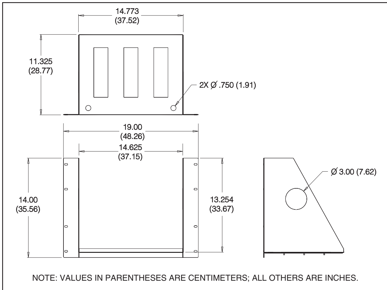
Figure 1. RMA131SU Dimension Drawing
