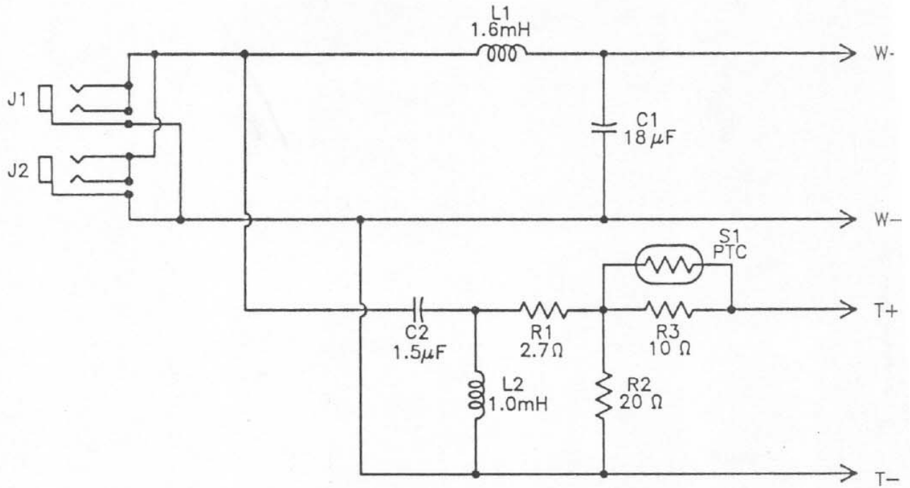
SCHEMATIC DIAGRAM
