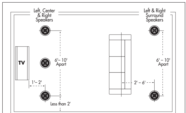
Figure 3: 5.1-Channel Home Theater Speaker Placement
