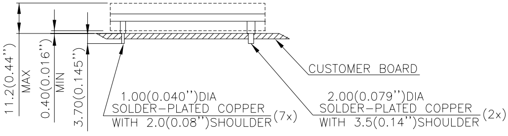
SIDE VIEW
