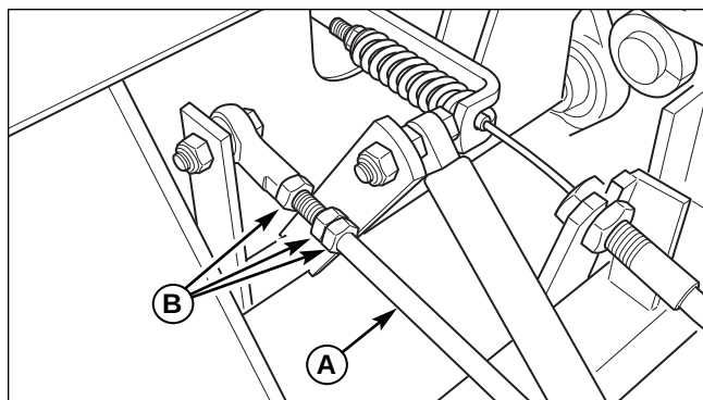
Figure 33. Neutral Adjustment (RH side shown) A. Adjustment Linkage Rod B. Nuts
