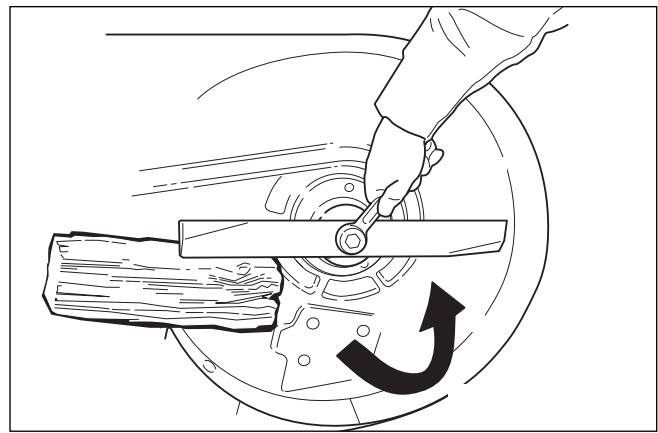
Figure 24. Loosening the Mower Blade for Removal
