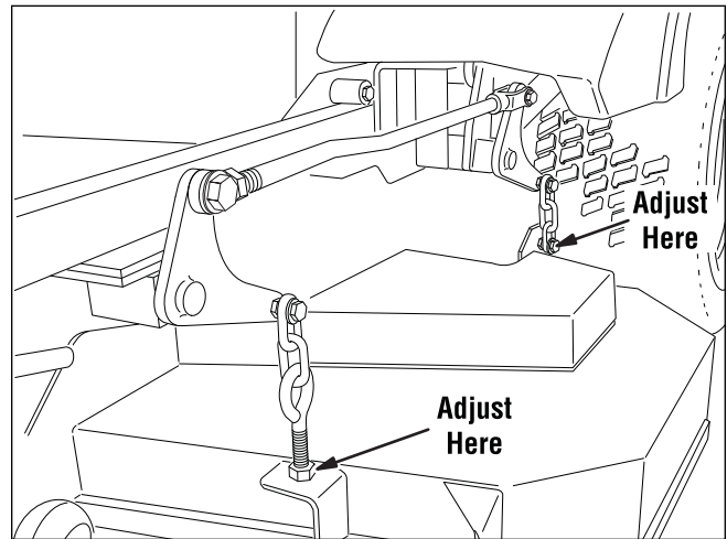
Figure 44. Adjust Lift Rod Timing
