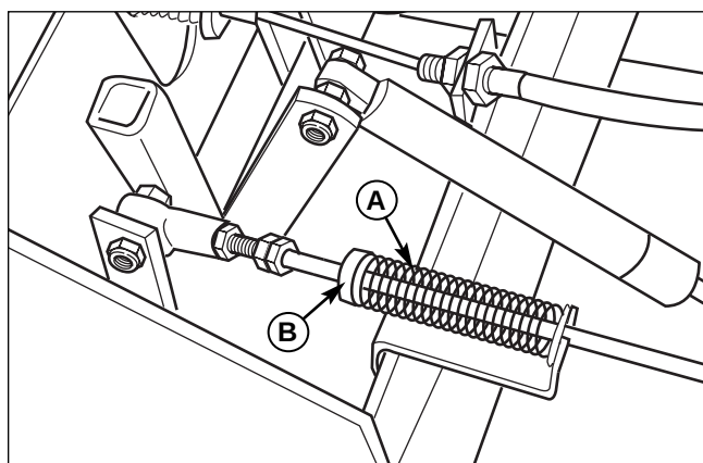
Figure 34. Return to Neutral Adjustment A. Return Spring B. Set Collar
