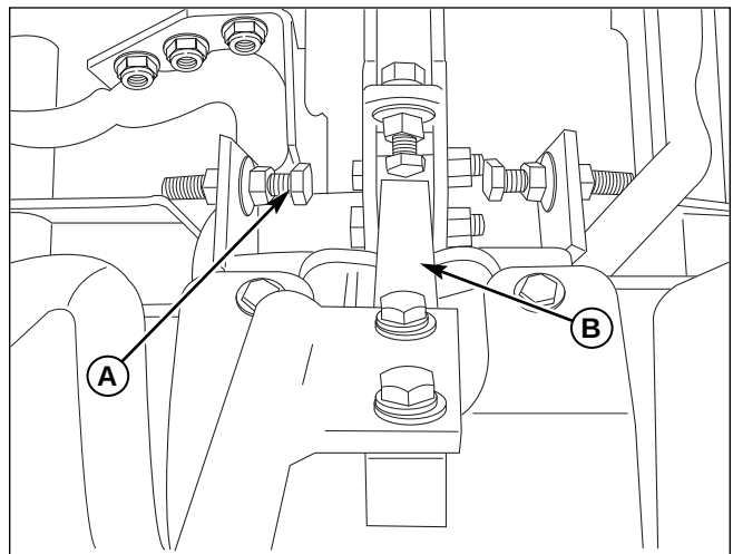
Figure 32. Top Speed Adjustment A. Top Speed Adjustment Bolt B. Control Lever Base
