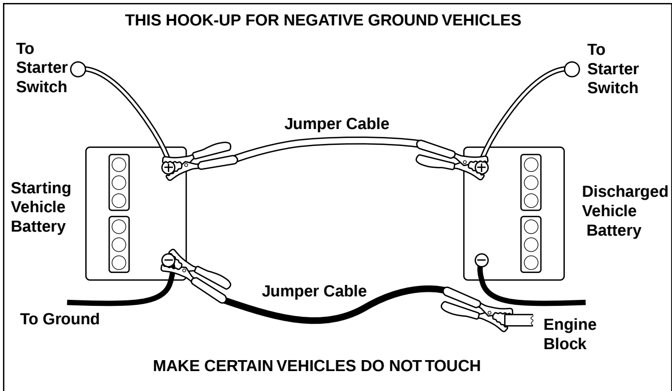
Figure 49. Jump Starting
