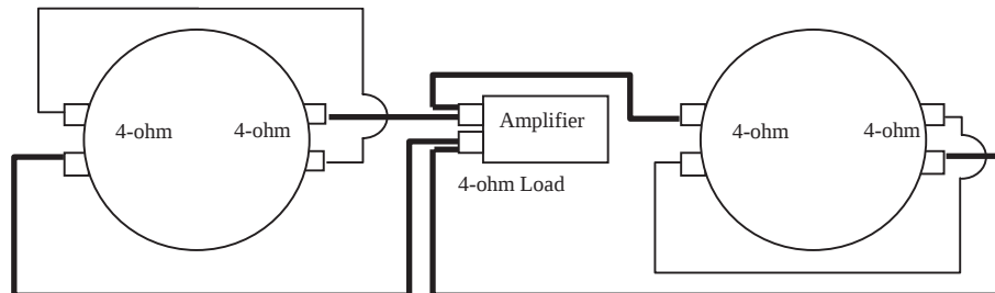
Series/Parallel voice coil configuration
