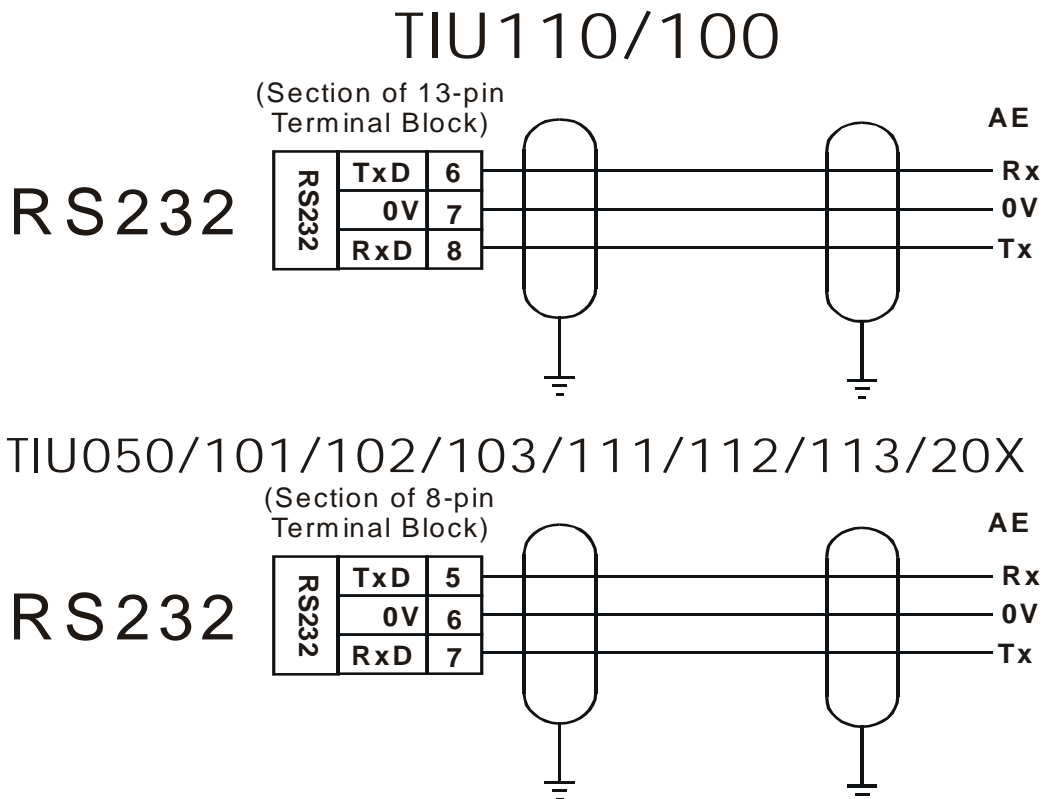
Figure 6.2 – RS-232 Connection
