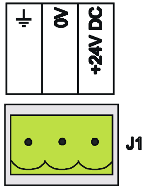
Figure 3.6 – Power Connector Powered by +24VDC and Ground.
