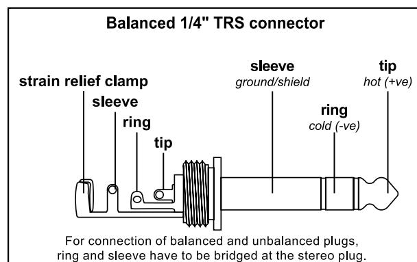
Fig. 4.1: 1/4" TRS connector
