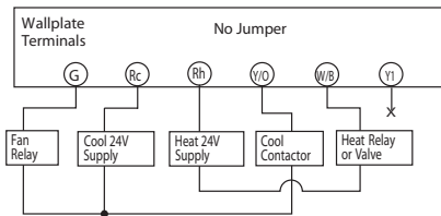
5-wire Heat/Cool System
