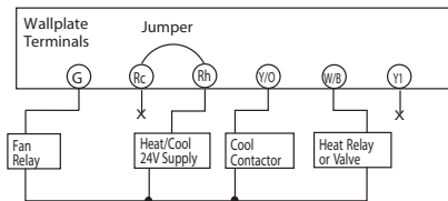
4-wire Heat/Cool System
