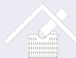
Installation en coin (vue de dessus) Corner installation (top view)
